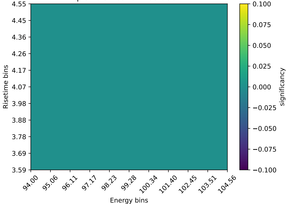
pion distribution 100.0GeV
